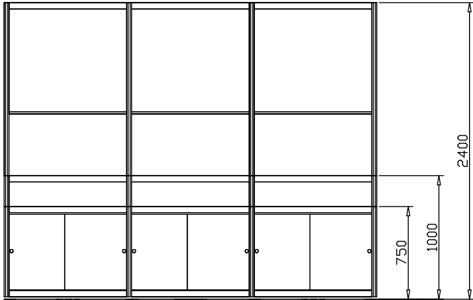
Elevation Plan
